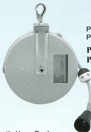
PU Automatic Hose Reel Plastic Housing \varnothing 200 mm \times 60 mm
