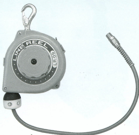
PU Air Hose Balancer Hose size: \varnothing 5.0 mm \times \varnothing 8.0 mm \times 1.2M.
