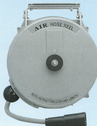
PVC Net Reinforced Automatic Hose Reel Plastic Housing \varnothing 275 mm \times 105 mm
